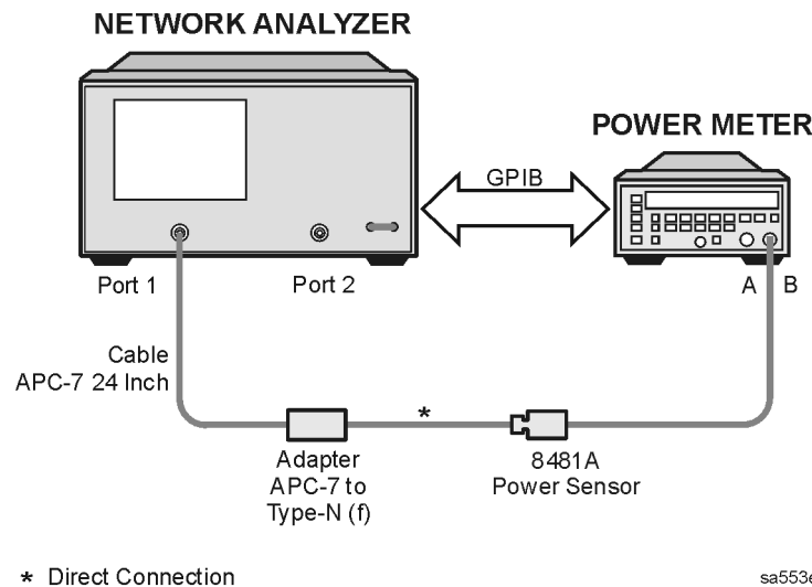
Figure 2-24 Setup for Power Meter Calibration on Test Port 1
