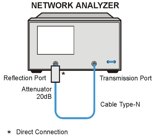
Figure 2-60 Output Power Linearity Test Setup
