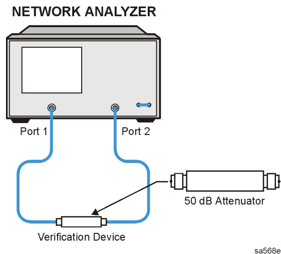
Figure 2-5 Connections for the 50 dB Verification Device
