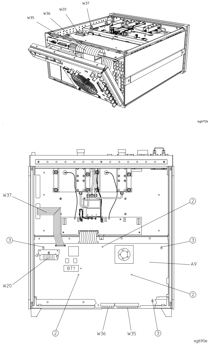
Figure 14-11 A9 CPU Board
