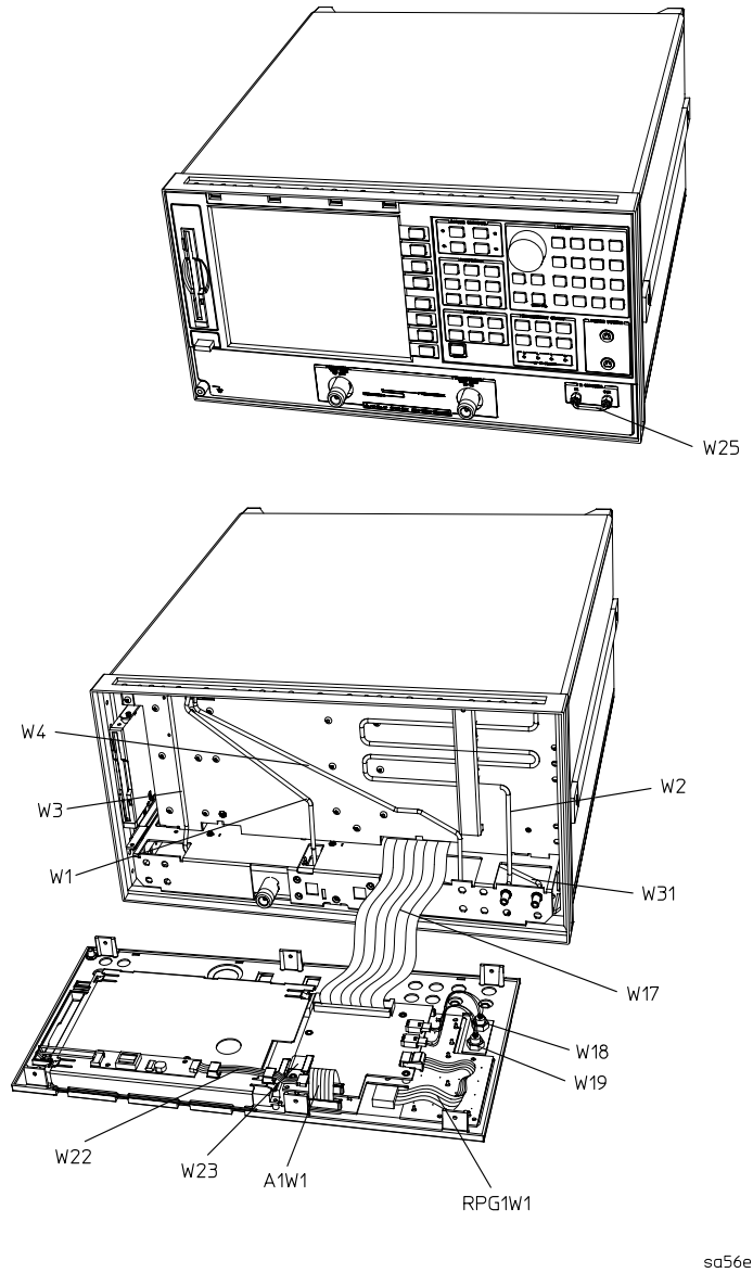
Figure 13-12 8753ET: Cables, Front
