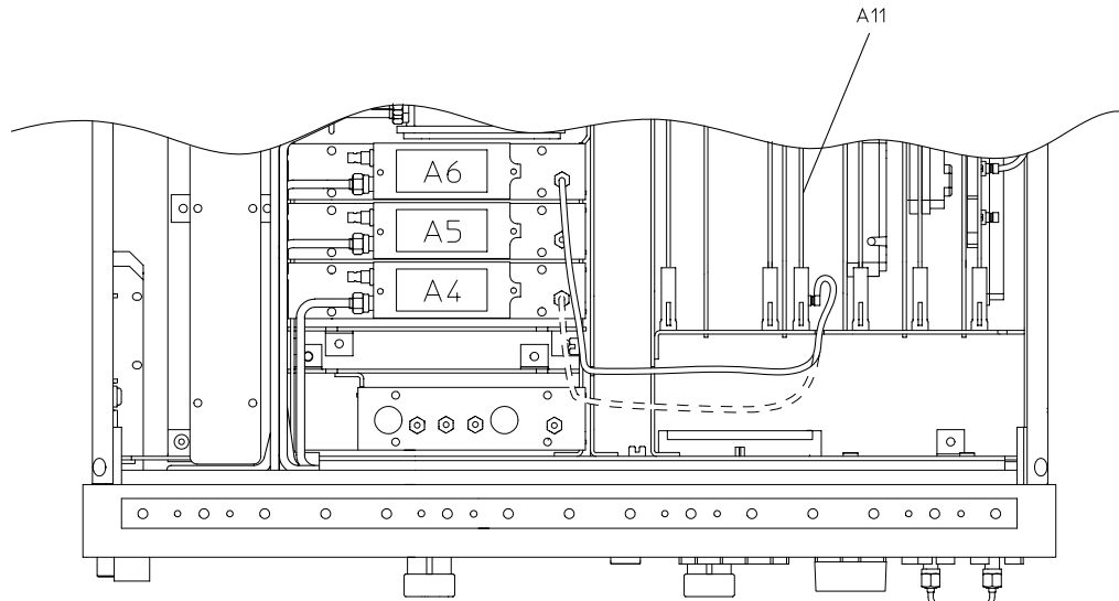
Figure 2-15 Connections for Substituting the R Sampler (A4)
