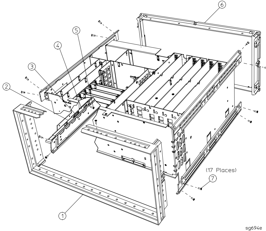
Figure 14-15 A17 Motherboard and Card Cage Assembly
