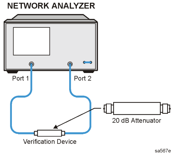
Figure 2-4 Connections for the 20 dB Verification Device
