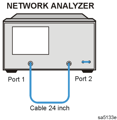
Figure 2-33 System Trace Noise Test Setup
