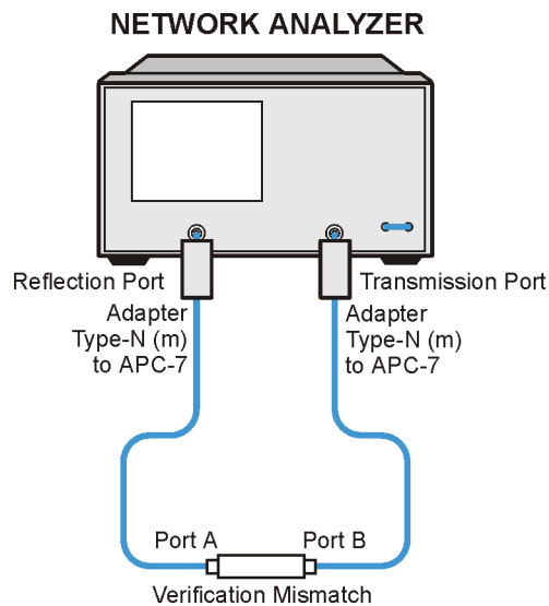
Figure 2-54 Mismatch Device Verification Setup 1
