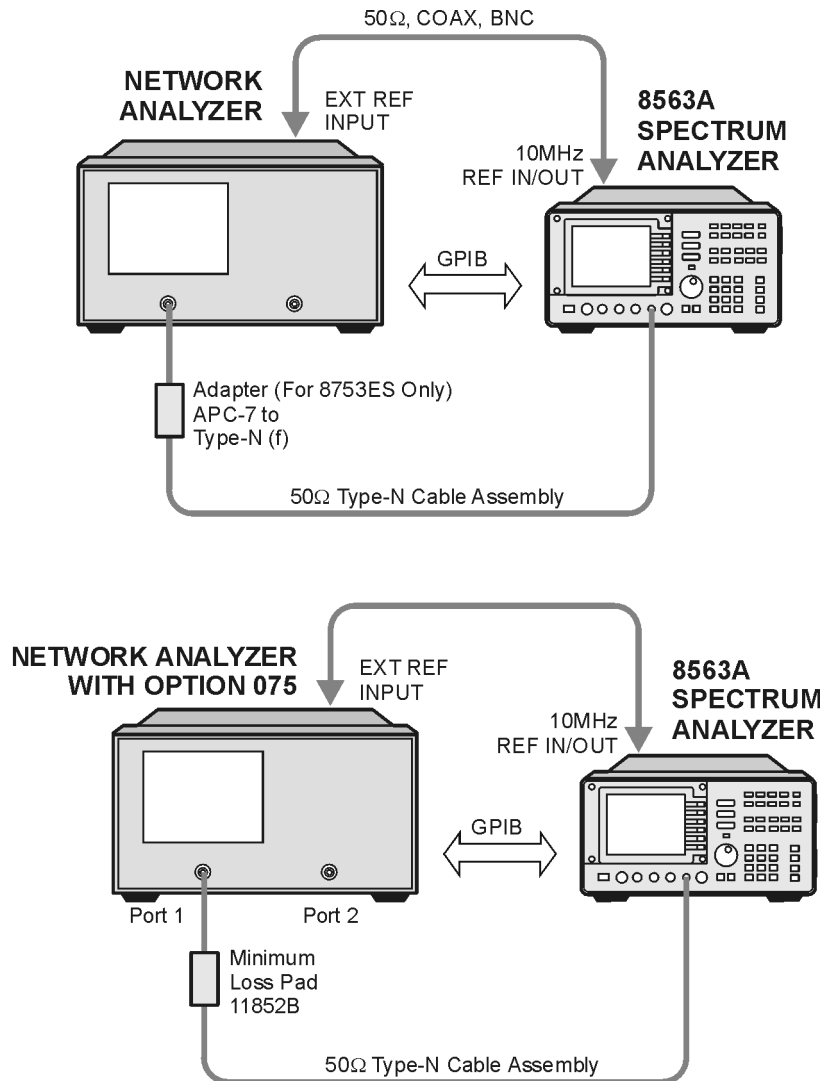
Figure 3-22 Fractional-N Spur Avoidance and FM Sideband Adjustment Setup
