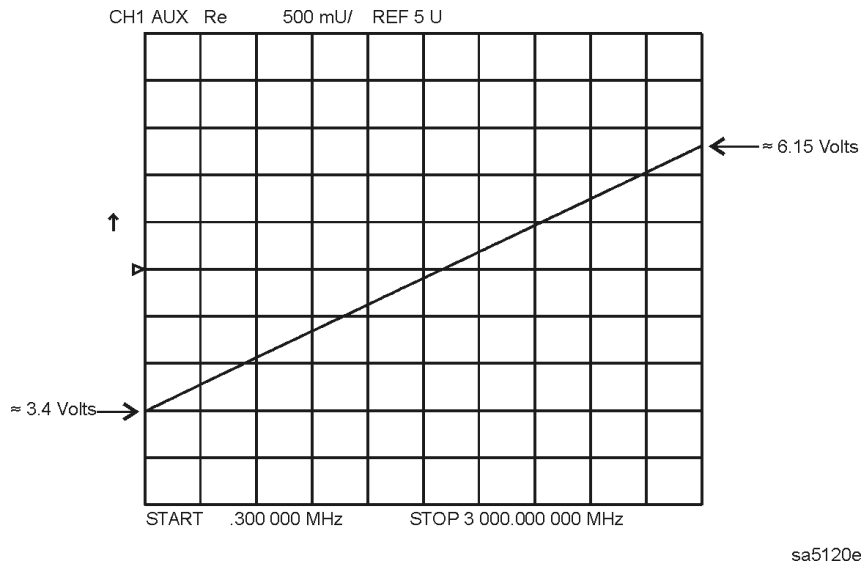
Figure 4-6 ABUS Node 16: 1 V/GHz
